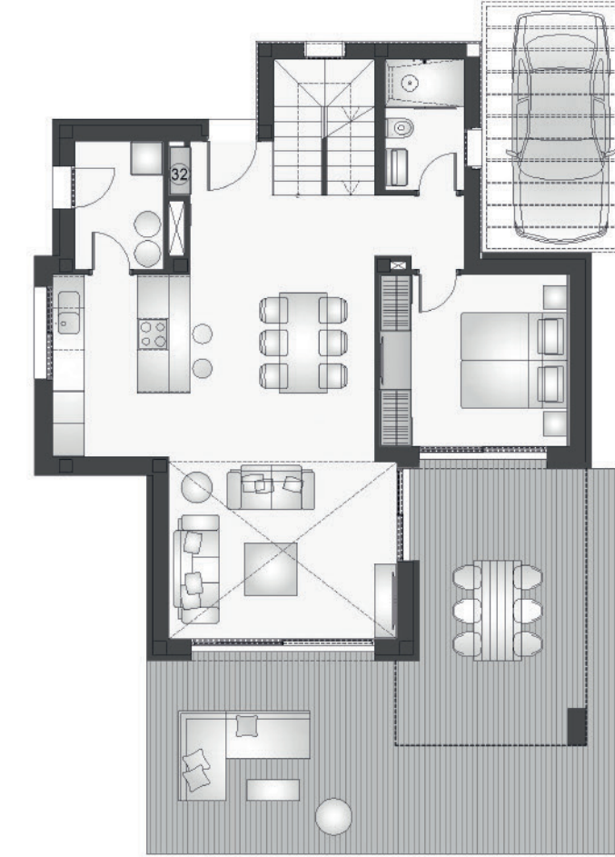
Planta Baja / Ground Floor
